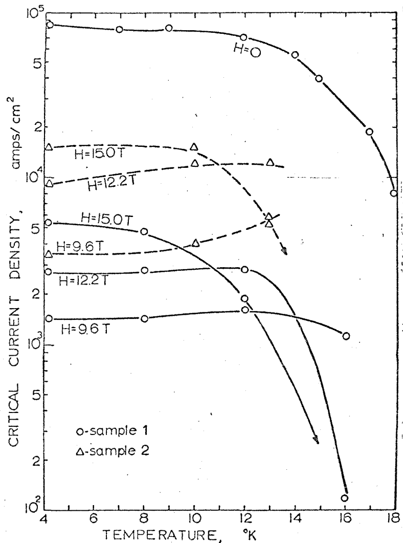
Fig. 1. J_c vs T at various applied transverse fields, for two specimens. Specimen No. 1 was annealed for 100 h at 725^{\circ}\text{C} and should have a higher T_c (by about 1.5^{\circ} ) than Specimen No. 2, which was not annealed.
